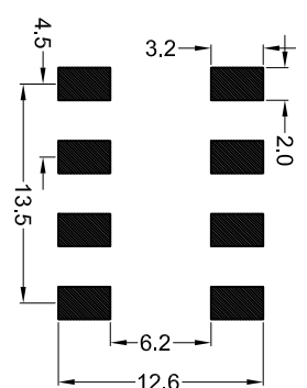
PCB LAYOUT
