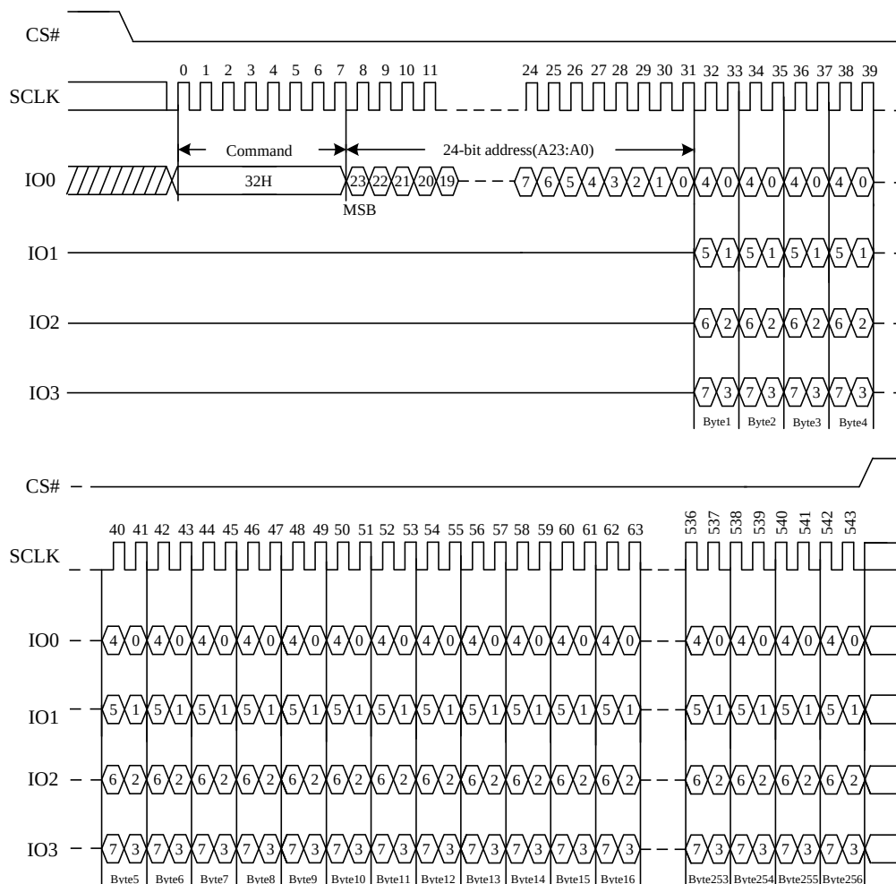
Figure 38. Quad Page Program Sequence Diagram
