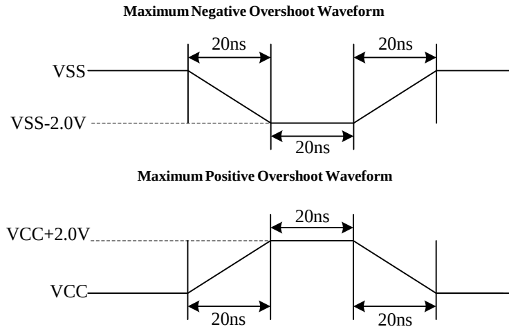
Figure 94. Input Test Waveform and Measurement Level
