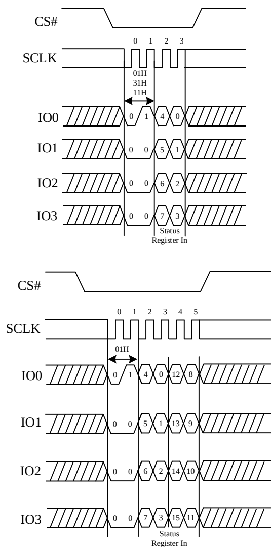
Figure 4. Write Status Register Sequence Diagram (QPI)
