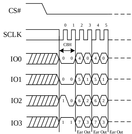
Figure 6. Read Extended Address Register Diagram (QPI)
