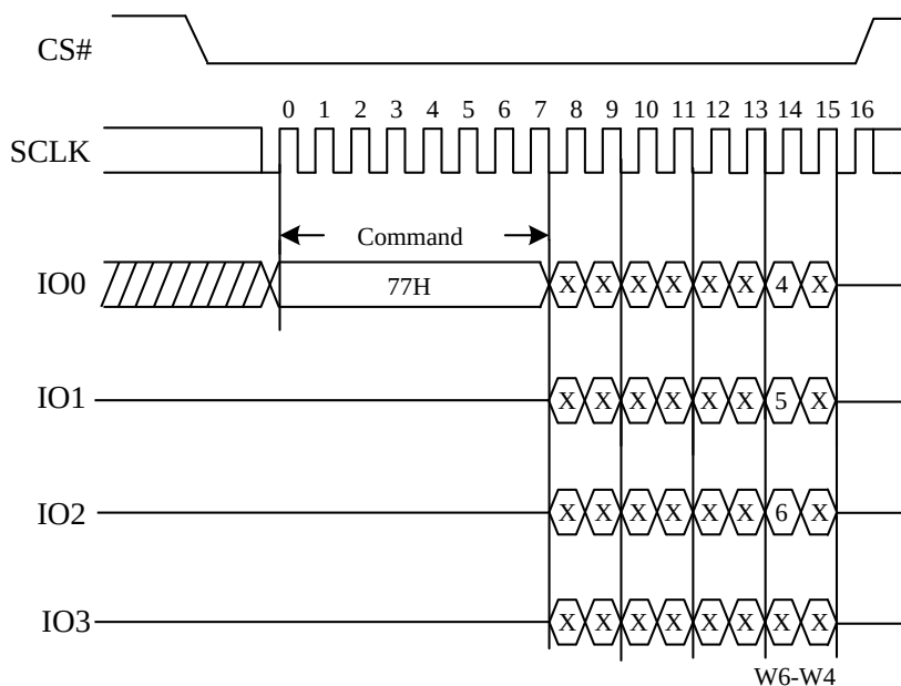
Figure 62. Set Burst with Wrap Sequence Diagram
