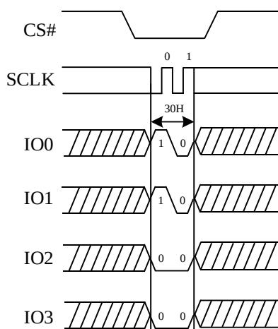
Figure 69. Clear Status Register Flags Sequence Diagram (QPI)
