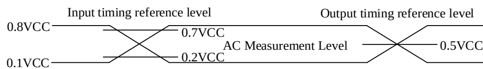
Figure 95. Absolute Maximum Ratings Diagram
