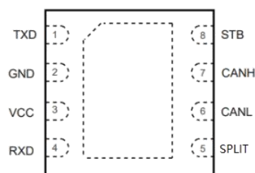
DFN-8 3*3
