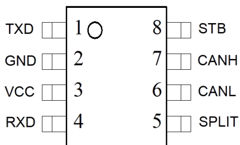
SOP-8/MSOP-8
