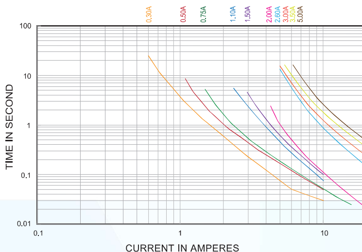
Average Time-Current Curve
