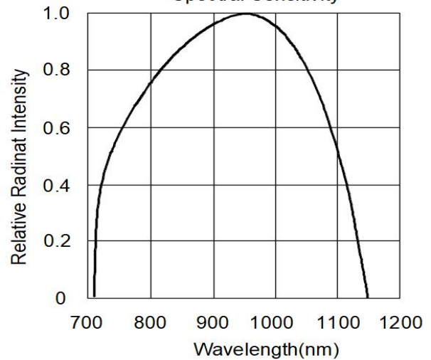
Spectral Sensitivity
