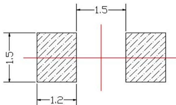
建议焊盘尺寸: Recommended Soldering Pattern
