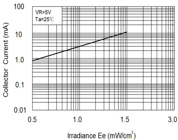
Collector Current vs. Irradiance
