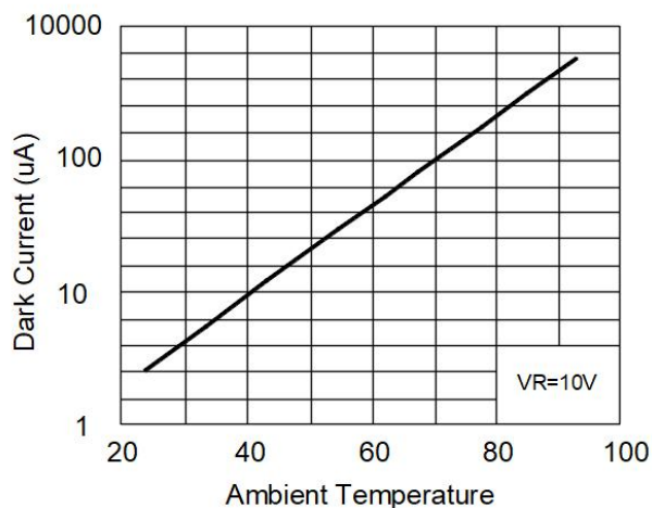
Dark Current vs. Ambient Temperature
