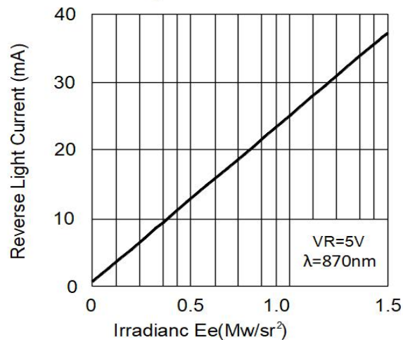
Reverse Light Current vs. Irradiance
