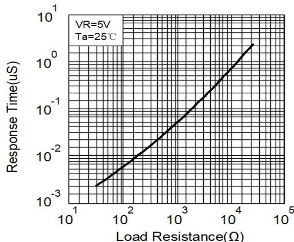
Response Time vs. Load Resistance
