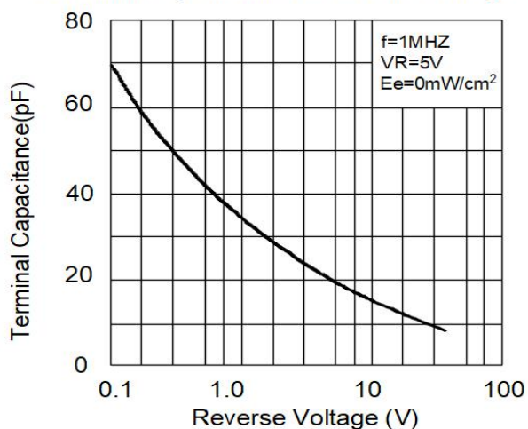
Terminal Capacitance vs. Reverse Voltage
