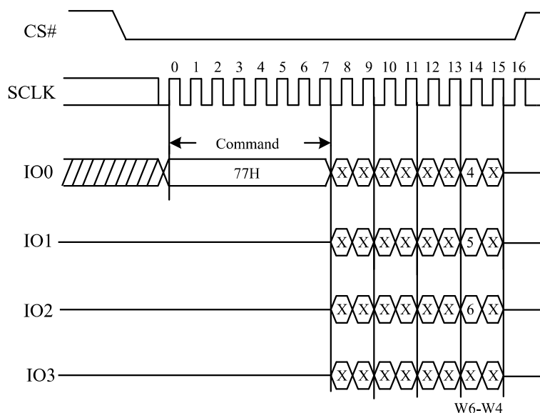
Figure 62. Set Burst with Wrap Sequence Diagram
