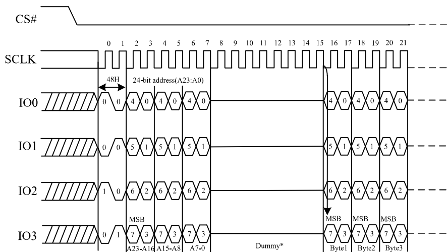
Figure 82. Read Security Registers command Sequence Diagram (QPI)
