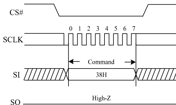
Figure 60. Enable QPI mode command Sequence Diagram
