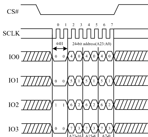
Figure 78. Erase Security Registers command Sequence Diagram (QPI)
