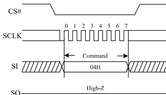
Figure 54. Write Disable Sequence Diagram
