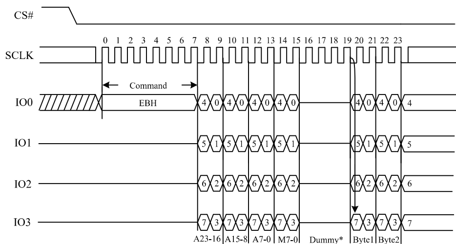
Figure 24. Quad I/O Fast Read Sequence Diagram (M5-4≠(1,0))
