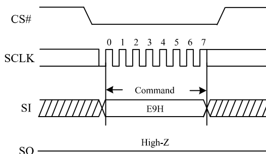
Figure 66. Disable 4-byte Mode Sequence Diagram (SPI)
