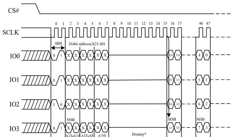
Figure 14. Read Unique ID (RUID) Sequence (QPI)
