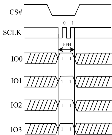
Figure 61. Disable QPI mode command Sequence Diagram (QPI)
