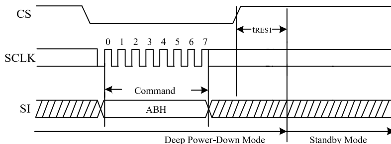
Figure 72. Release Power-Down Sequence Diagram
