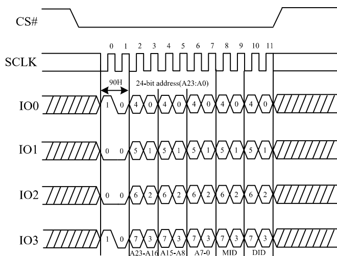
Figure 10. Read Manufacture ID/ Device ID Sequence Diagram (QPI)
