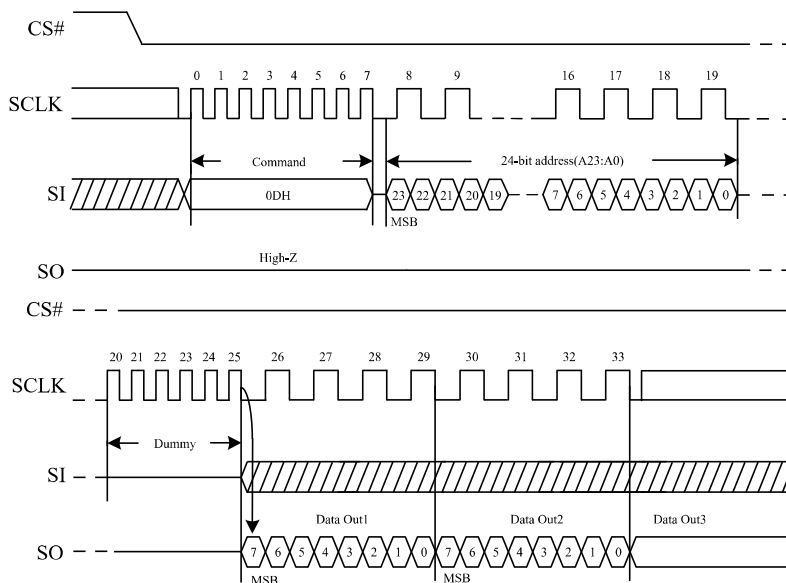
Figure 28. DTR Fast Read Instruction
