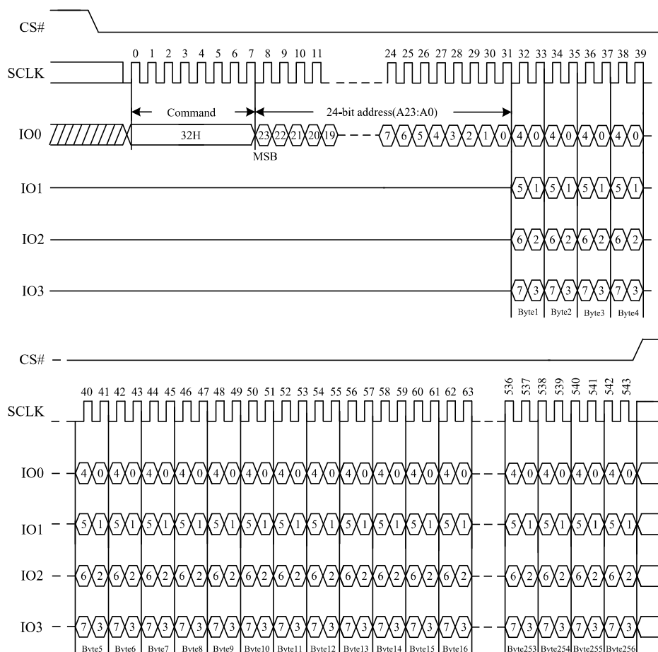
Figure 38. Quad Page Program Sequence Diagram
