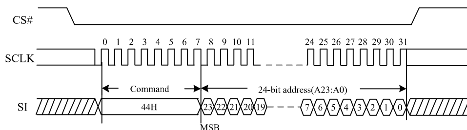
Figure 77. Erase Security Registers command Sequence Diagram
