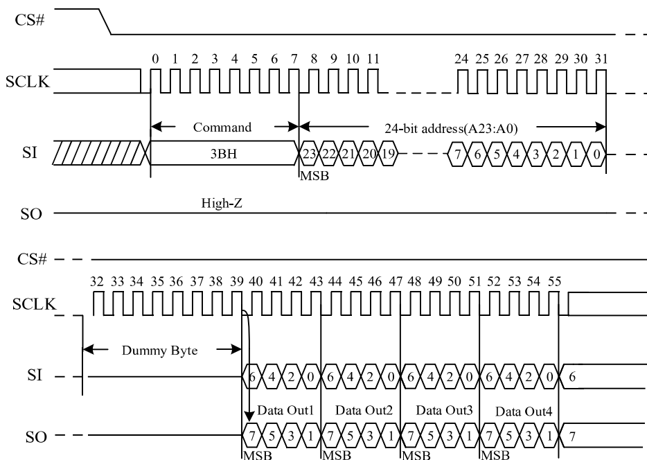
Figure 20. Dual Output Fast Read Sequence Diagram
