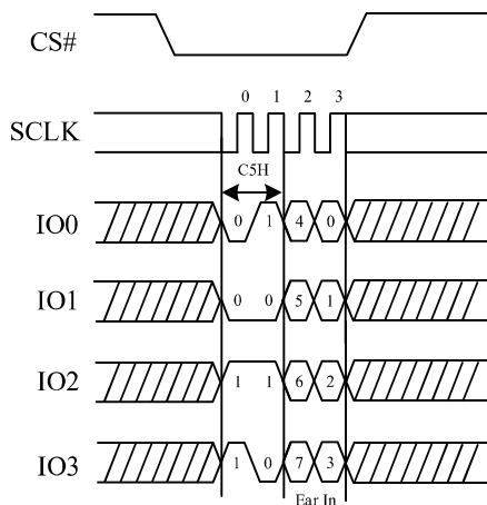
Figure 8. Write Extended Address Register Diagram (QPI)
