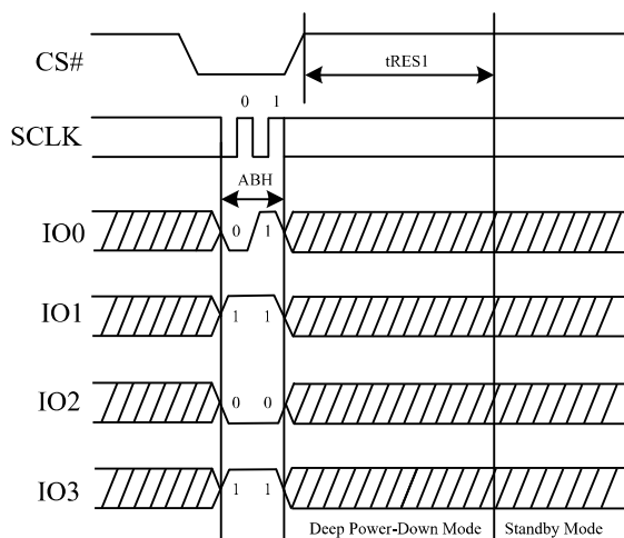
Figure 73. Release Power-Down Sequence Diagram (QPI)
