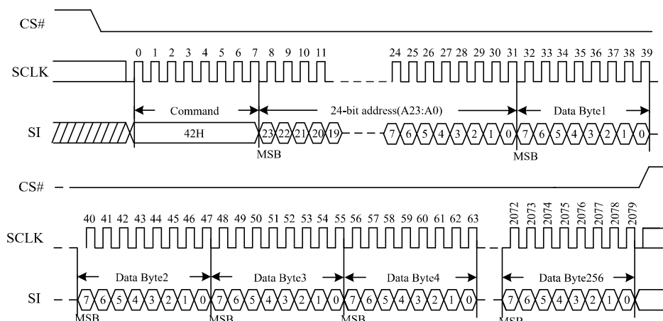
Figure 79. Program Security Registers command Sequence Diagram
