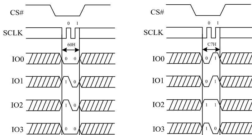
Figure 47. Chip Erase Sequence Diagram (QPI)
