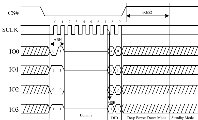
Figure 75. Release Power-Down/Read Device ID Sequence Diagram (QPI)
