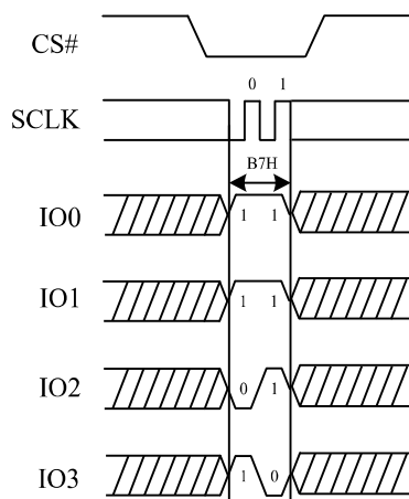
Figure 65. Enable 4-byte Mode Sequence Diagram (QPI)
