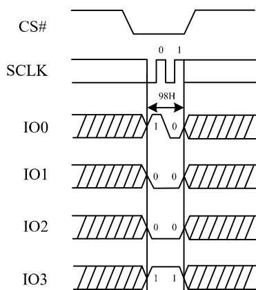
Figure 86. The Global Block/Sector Unlock Sequence Diagram (QPI)
