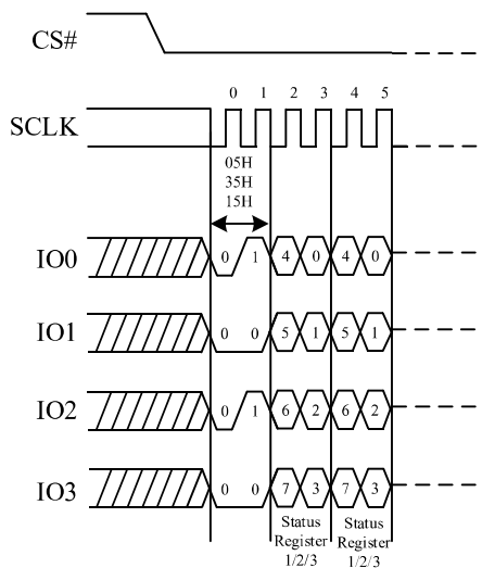
Figure 2. Read Status Register Sequence Diagram (QPI)
