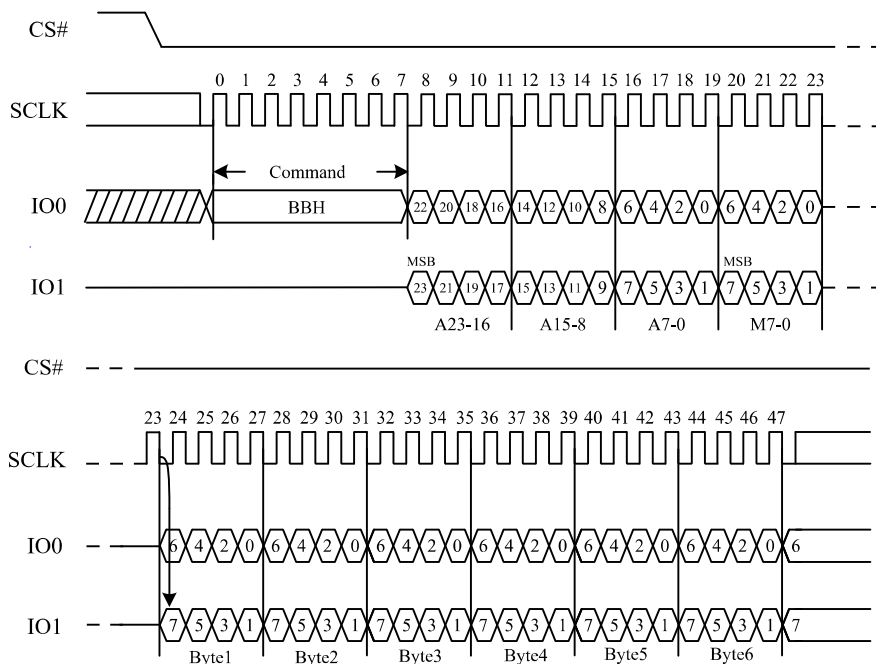
Figure 21. Dual I/O Fast Read Sequence Diagram (M5-4≠(1,0))
