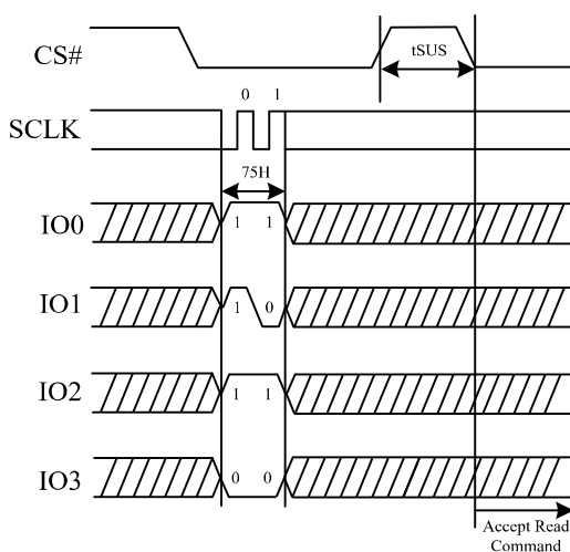
Figure 57. Program/Erase Suspend Sequence Diagram (QPI)
