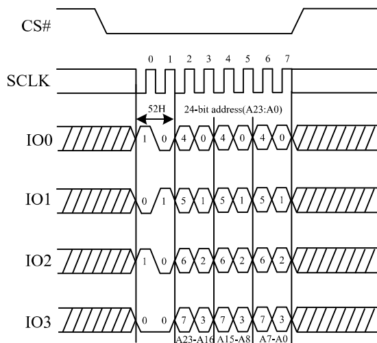
Figure 43. 32KB Block Erase Sequence Diagram (QPI)
