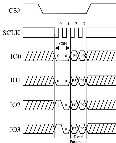
Figure 63. Set Read Parameters command Sequence Diagram (QPI)
