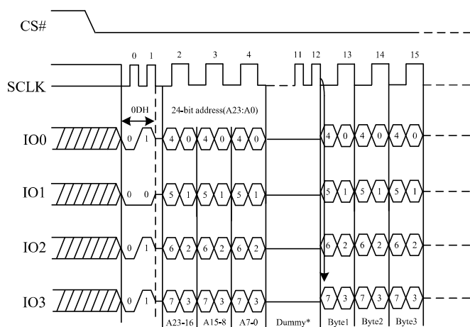
Figure 29. DTR Fast Read Instruction (QPI)
