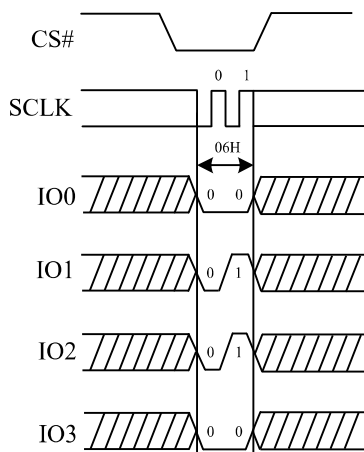
Figure 51. Write Enable Sequence Diagram (QPI)
