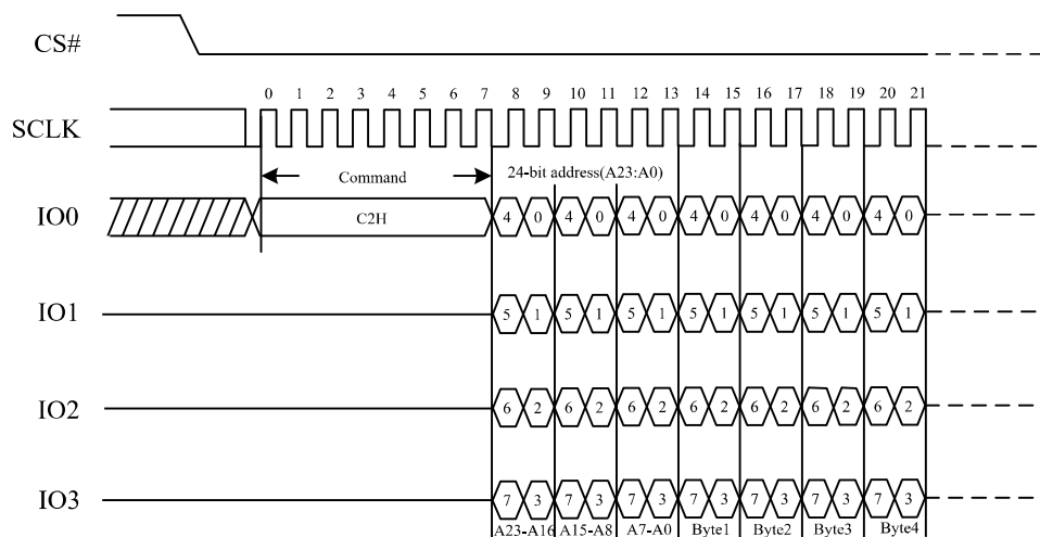
Figure 39. Quad Page Program Sequence Diagram
