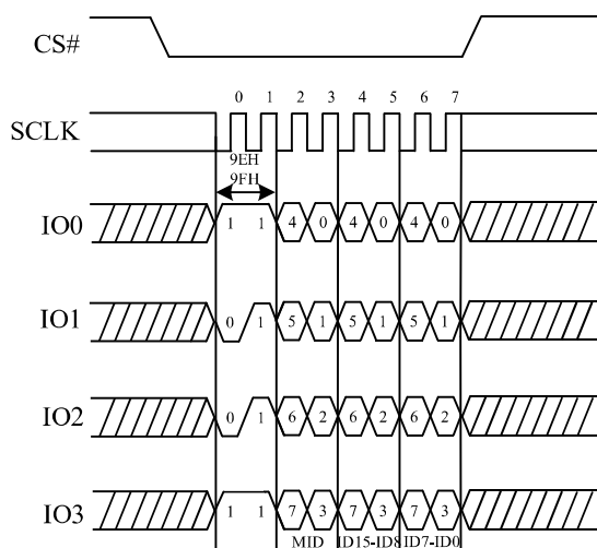
Figure 16. Read Identification ID Sequence Diagram (QPI)
