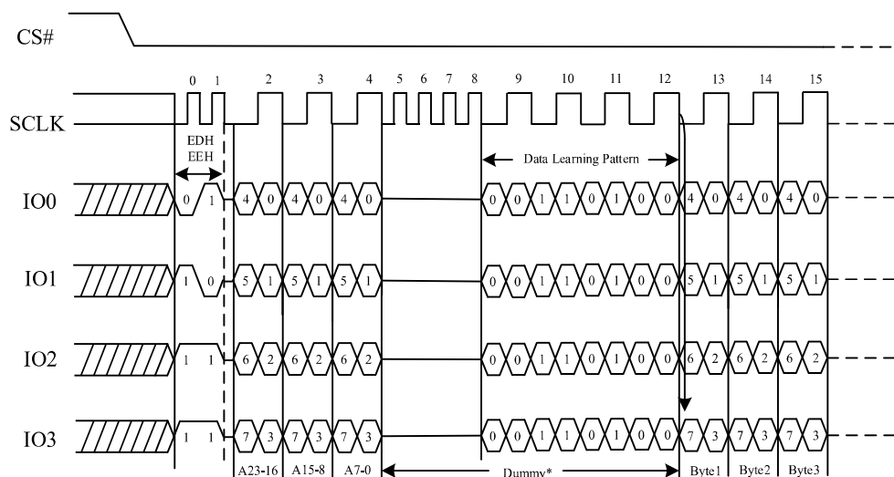
DLP Sequence Diagram (QPI)
