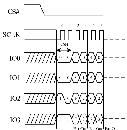
Figure 6. Read Extended Address Register Diagram (QPI)
