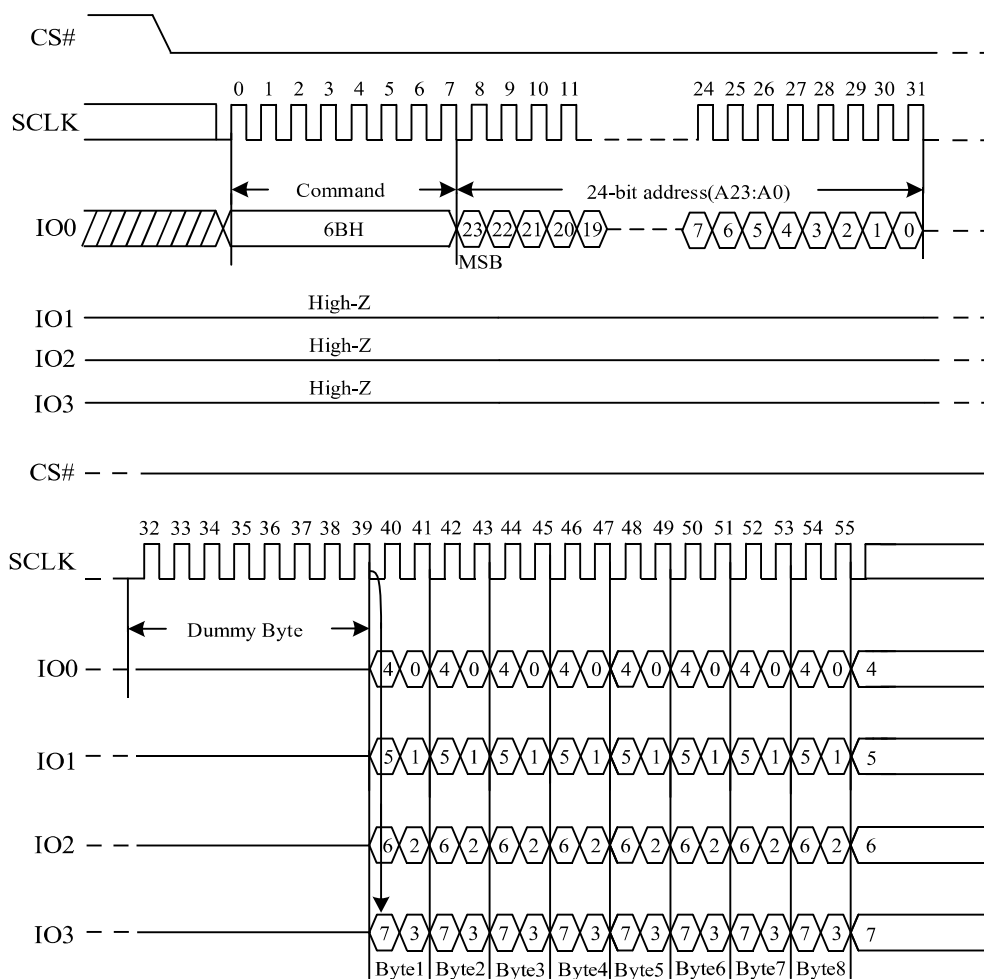
Figure 23. Quad Output Fast Read Sequence Diagram
