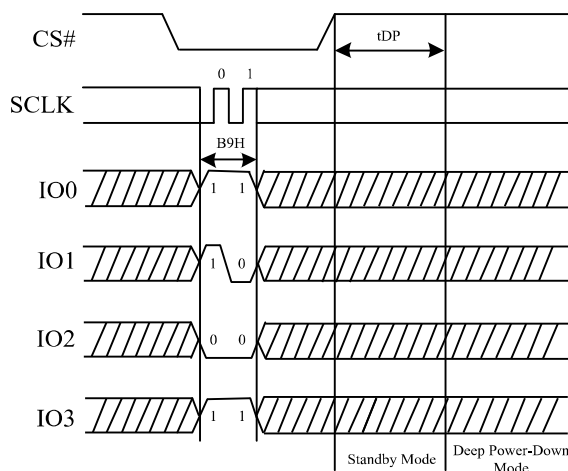
Figure 71. Deep Power-Down Sequence Diagram (QPI)
