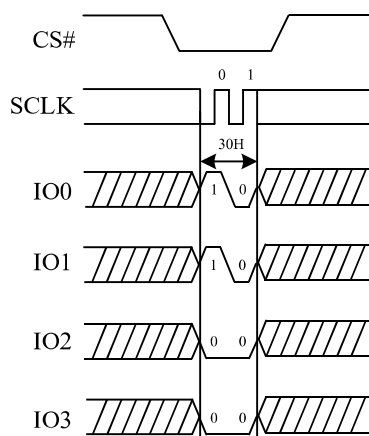
Figure 69. Clear Status Register Flags Sequence Diagram (QPI)
