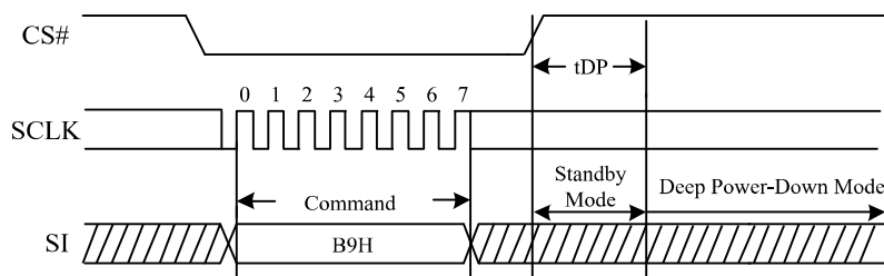
Figure 70. Deep Power-Down Sequence Diagram
