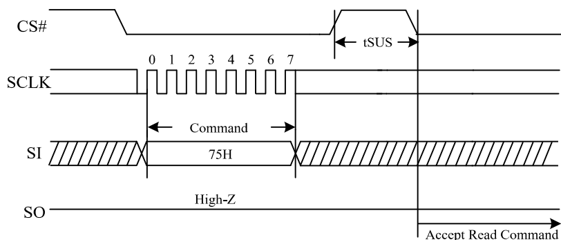
Figure 56. Program/Erase Suspend Sequence Diagram
