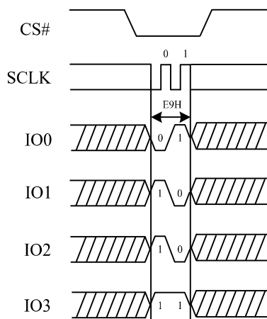
Figure 67. Disable 4-byte Mode Sequence Diagram (QPI)
