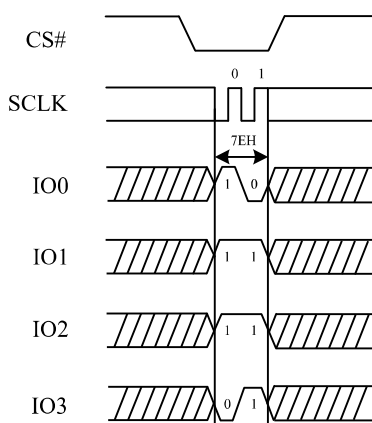
Figure 84. The Global Block/Sector Lock Sequence Diagram (QPI)
