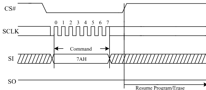
Figure 58. Program/Erase Resume Sequence Diagram
