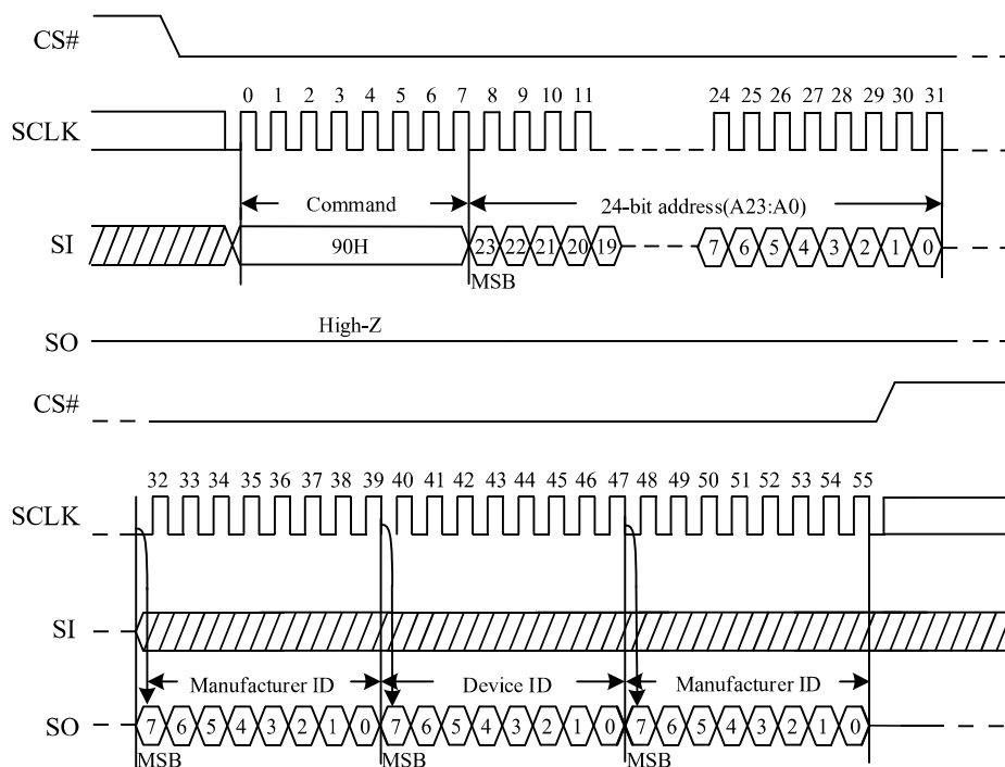
Figure 9. Read Manufacture ID/ Device ID Sequence Diagram
