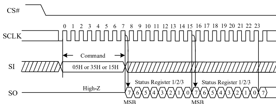
Figure 1. Read Status Register Sequence Diagram
