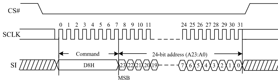
Figure 44. 64KB Block Erase Sequence Diagram
