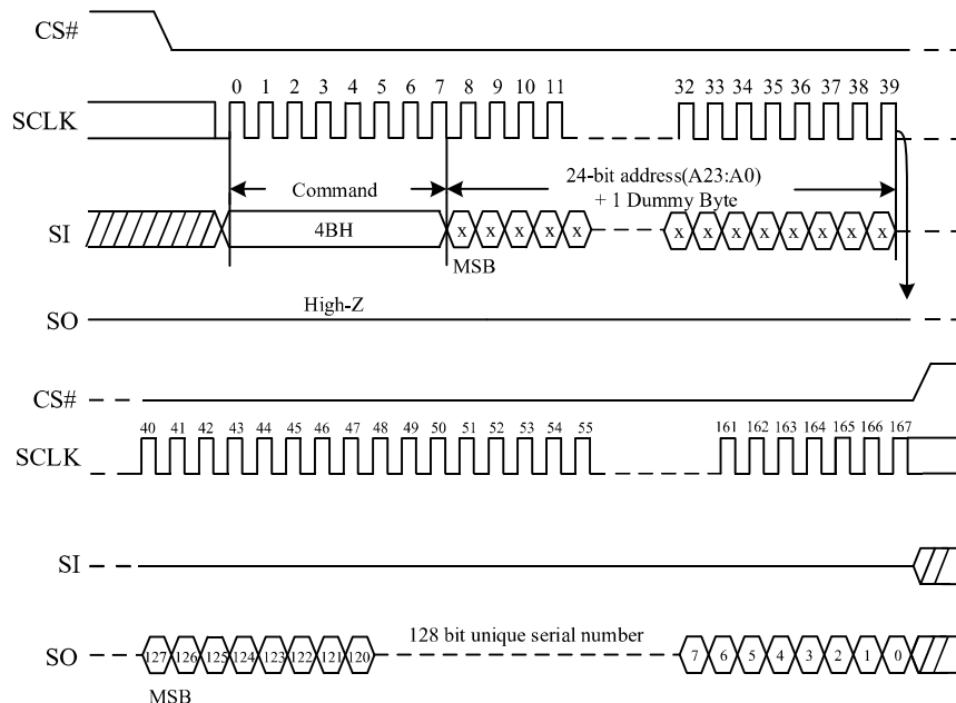
Figure 13. Read Unique ID (RUID) Sequence
