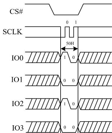
Figure 53. Write Enable for Volatile Status Register Sequence Diagram (QPI)
