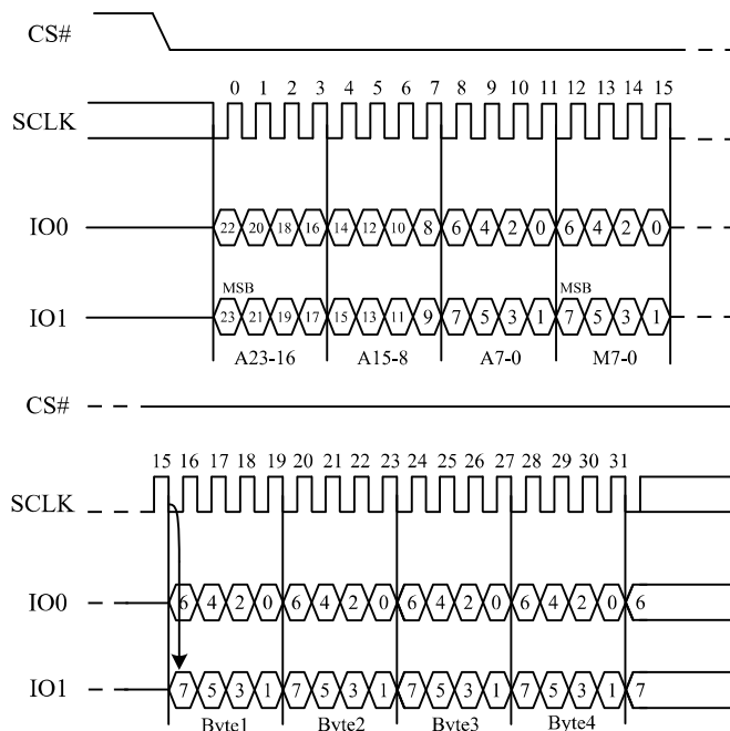
Figure 22. Dual I/O Fast Read Sequence Diagram (M5-4=(1,0))
