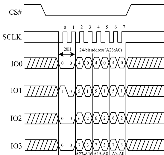
Figure 41. Sector Erase Sequence Diagram (QPI)
