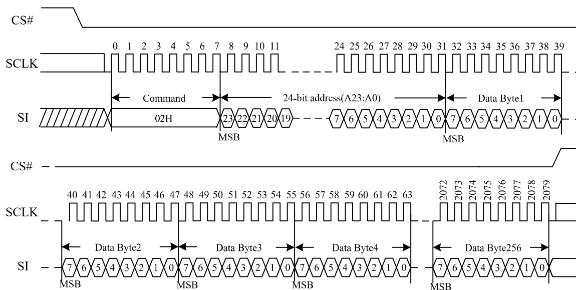
Figure 36. Page Program Sequence Diagram
