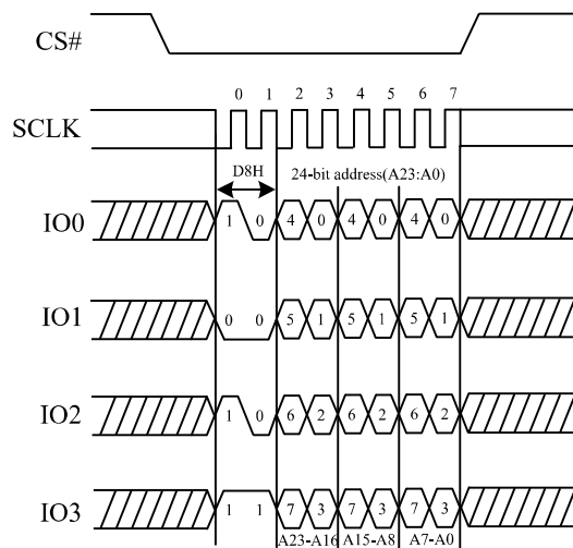
Figure 45. 64KB Block Erase Sequence Diagram (QPI)
