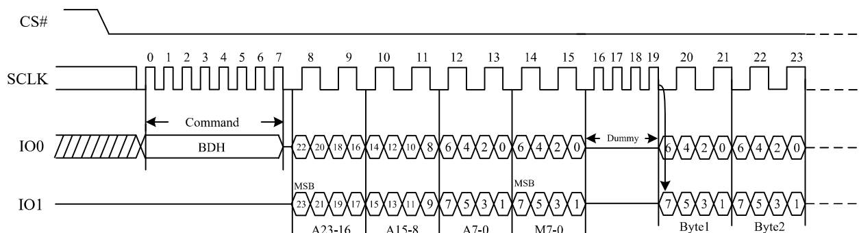
Figure 30. DTR Fast Read Dual I/O(Initial instruction or previous M5-4≠10, SPI Mode only)
