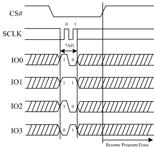
Figure 59. Program/Erase Resume Sequence Diagram (QPI)
