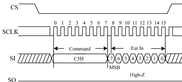
Figure 7. Write Extended Address Register Diagram
