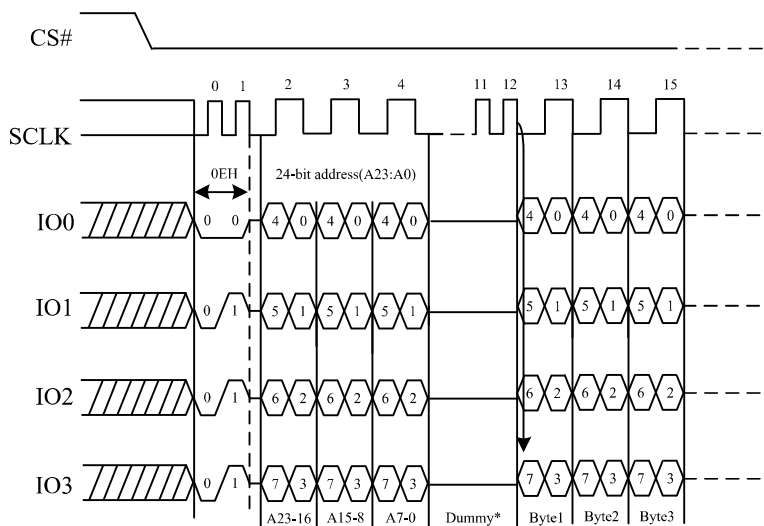
Figure 35. DTR Burst Read With Wrap command Sequence Diagram (QPI)
