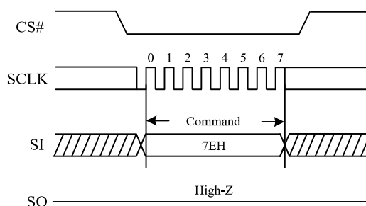
Figure 83. The Global Block/Sector Lock Sequence Diagram
