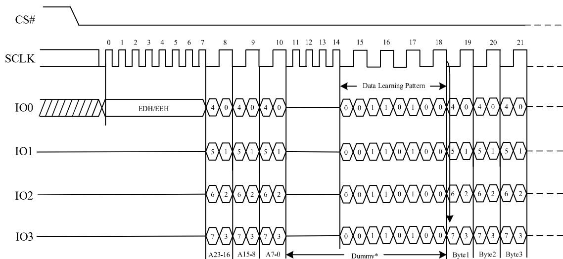
DLP Sequence Diagram
