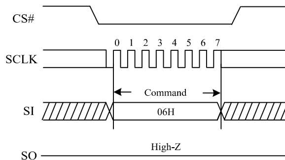
Figure 50. Write Enable Sequence Diagram
