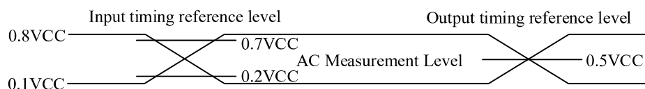
Figure 95. Absolute Maximum Ratings Diagram
