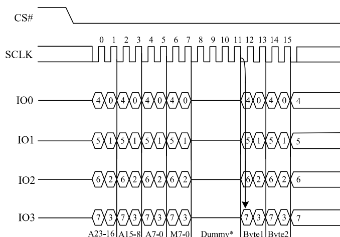
Figure 25. Quad I/O Fast Read Sequence Diagram (M5-4=(1,0))
