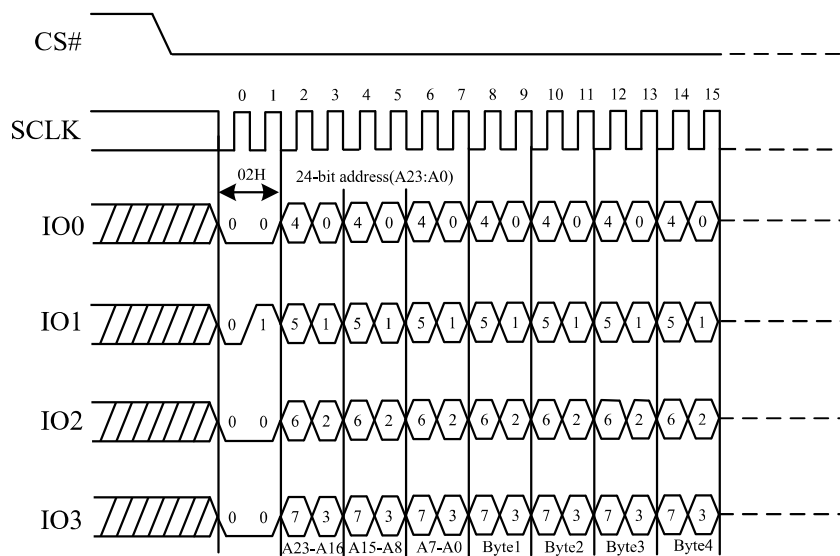
Figure 37. Page Program Sequence Diagram (QPI)
