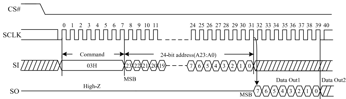
Figure 17. Read Data Bytes Sequence Diagram
