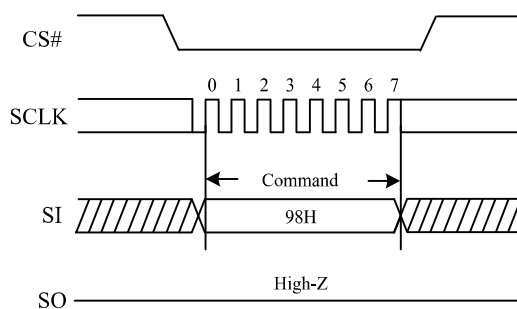
Figure 85. The Global Block/Sector Unlock Sequence Diagram
