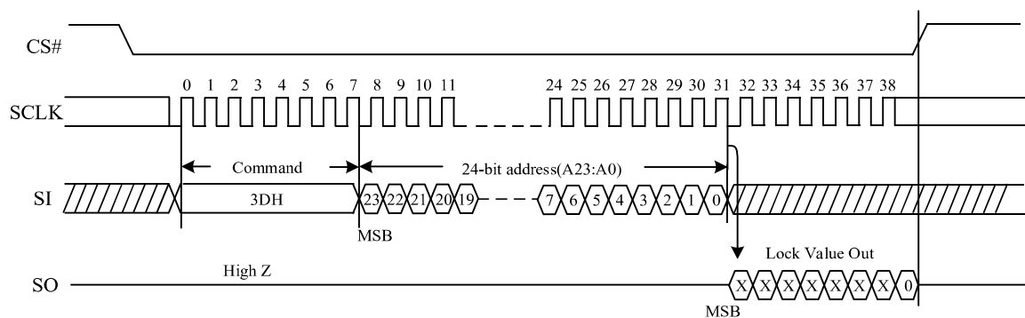
Figure 91. Read Individual Block/Sector lock command Sequence Diagram
