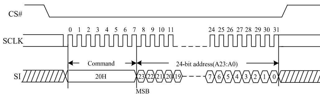
Figure 40. Sector Erase Sequence Diagram
