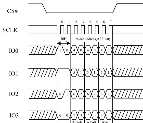
Figure 88. Individual Block/Sector Lock command Sequence Diagram (QPI)
