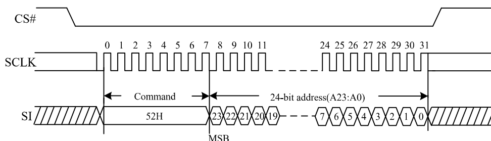
Figure 42. 32KB Block Erase Sequence Diagram
