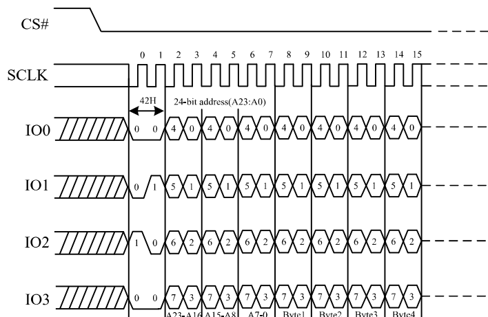
Figure 80. Program Security Registers command Sequence Diagram (QPI)
