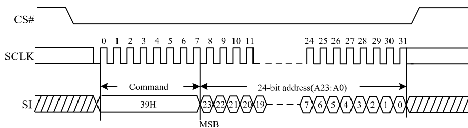
Figure 89. Individual Block/Sector Unlock command Sequence Diagram
