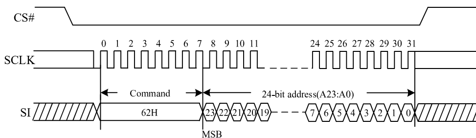
Figure 76. Program Strong Sequence Diagram
