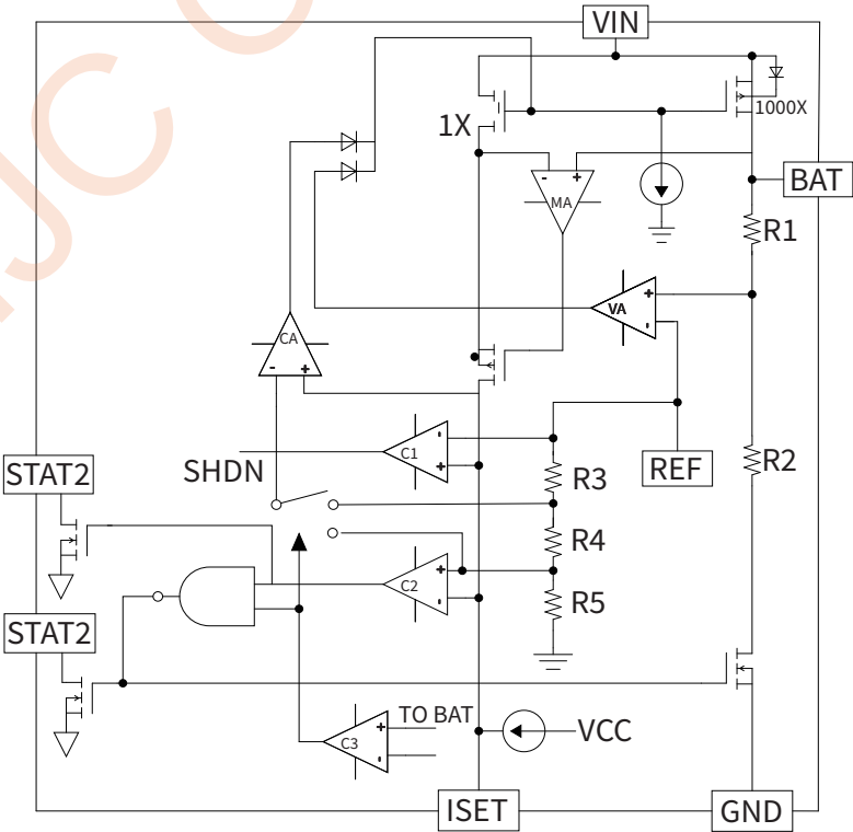
Figure 1.Internal Block Diagram
