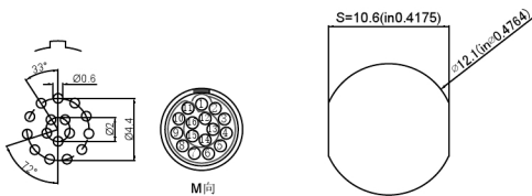
Pcb plate opening size (PCB板开孔尺寸)
