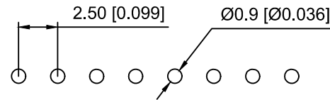
PCB Layout
