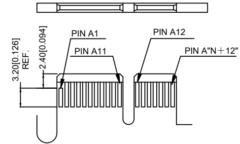
SECONDARY (SOLDER) SIDE PCI-E ADD-IN CARD EDGE-FINGER DIMENSION
