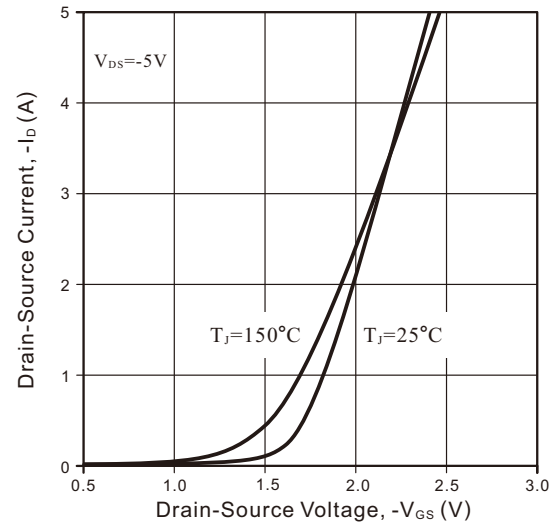
Fig2. Transfer Characteristic
