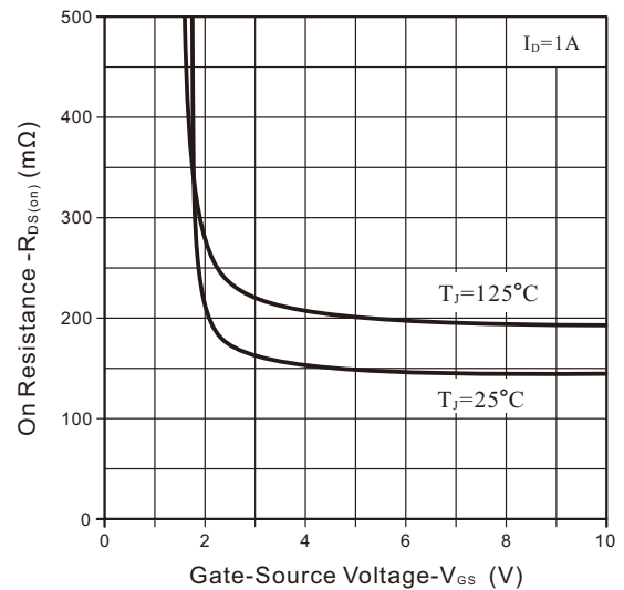
Fig4. On-Resistance vs. Gate-to-Source Voltage
