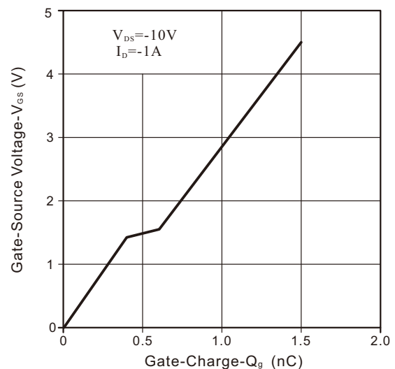
Fig6. Typical Gate-Charge
