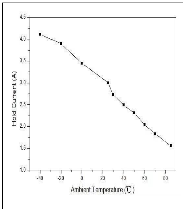
Thermal Derating Curve
