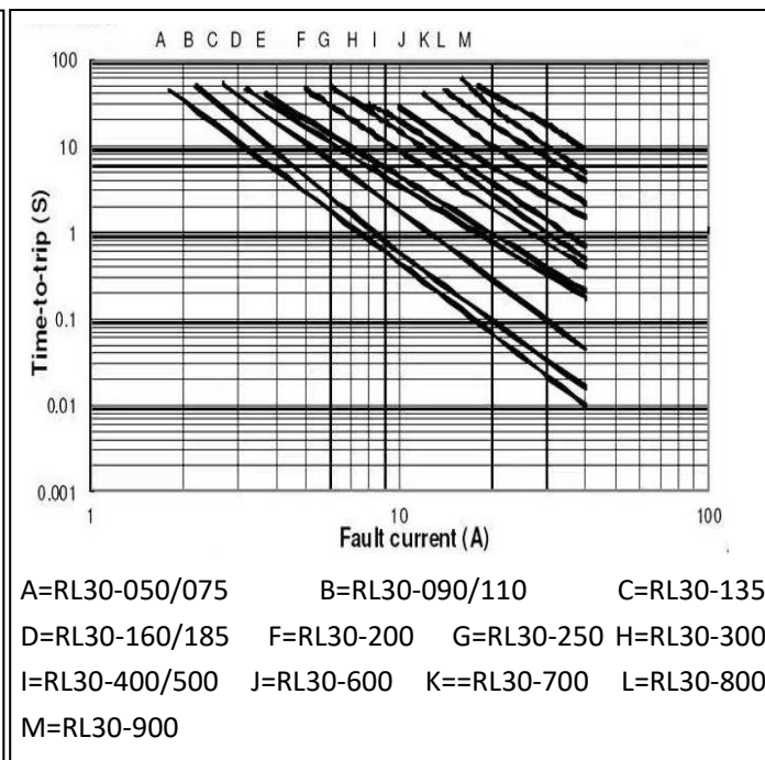
Average Time-Current Curve
