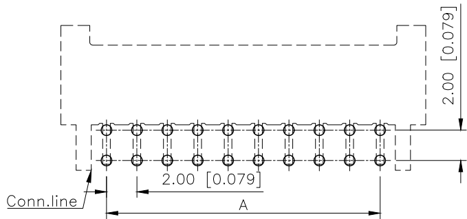
PCB LAYOUT
