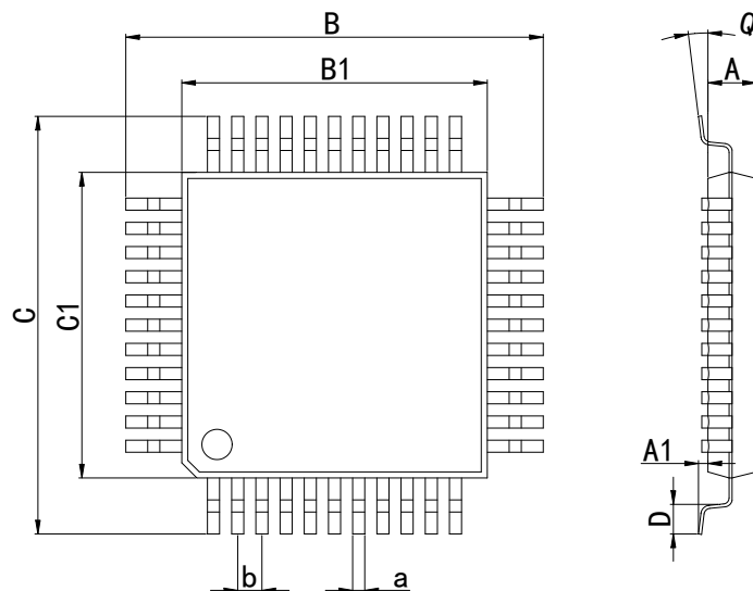
Dimensions In Millimeters(LQFP-44)
