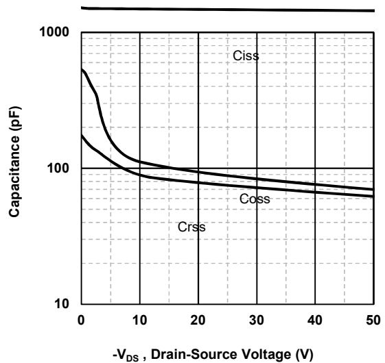
Fig6 Typical Capacitance Vs. Drain-Source
