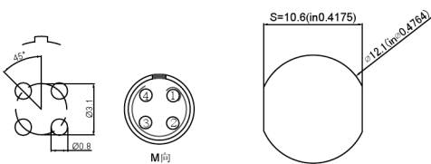
Pcb plate opening size (PCB板开孔尺寸)
