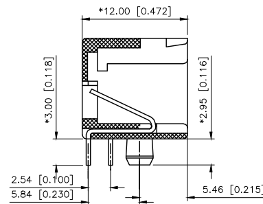
CUTAWAY VIEW
