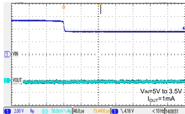
Line transient
