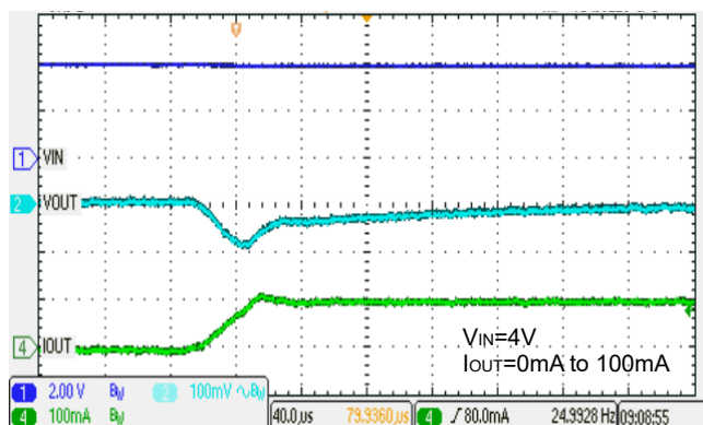
Load transient
