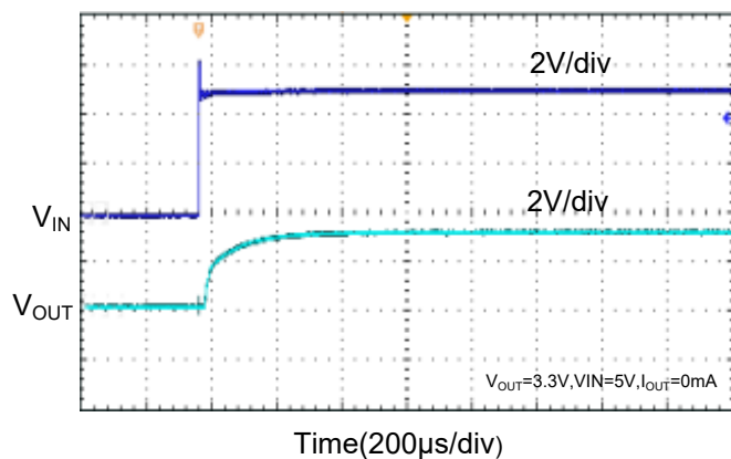
Power-on waveform
