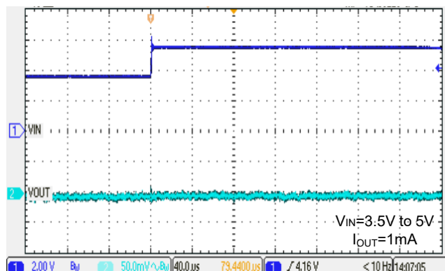
Line transient
