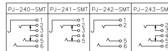
SCHEMATIC
