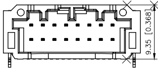
16 PIN
