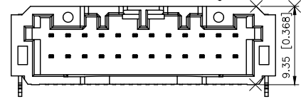
24 PIN
