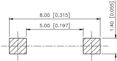
P.C.B MOUNTING HOLES
