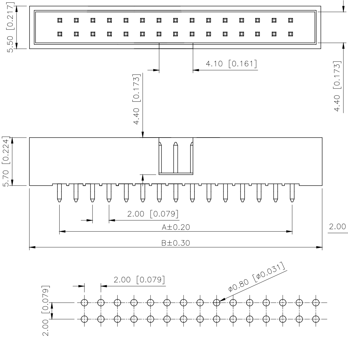
PCB LAYOUT
