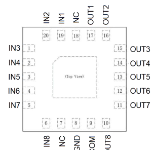
QFN-20 4*4
