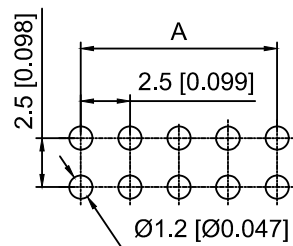
Recommended PCB Layout(Top view) Tolerance:±0.05mm
