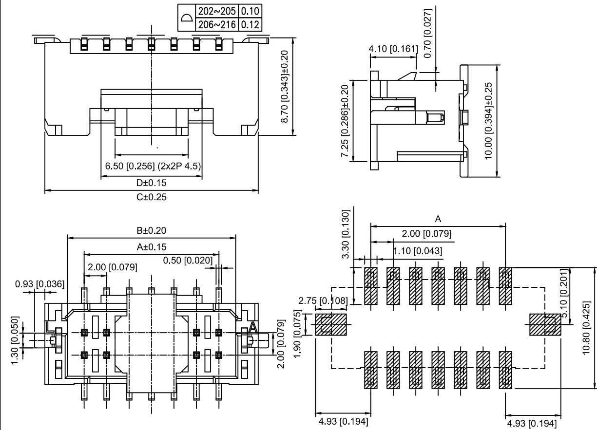
PCB LAYOUT(Tolerance:±0.05)
