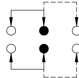
SCHEMATIC (NON-SHORTING)
