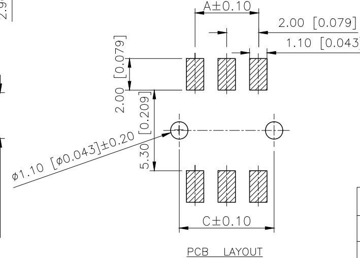
PCB LAYOUT
