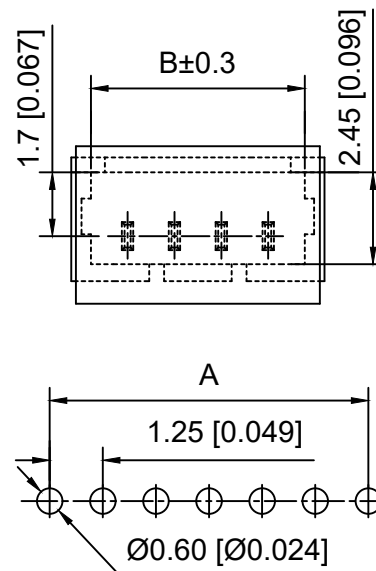
Recommended PCB Layout(Top view) Tolerance:±0.05mm
