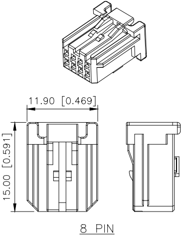
8 PIN
