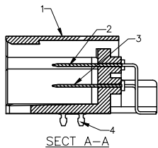
SECT. A-A
