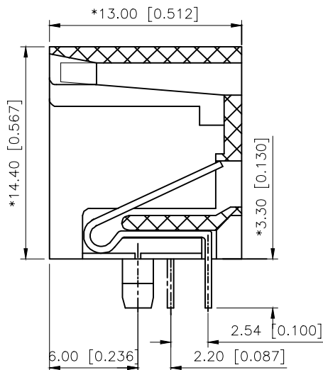
CUTAWAY VIEW
