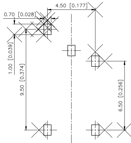
PCB_LAYOUT
