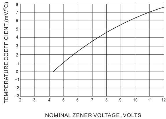
Fig.1 TEMPERATURE COEFFICIENTS
