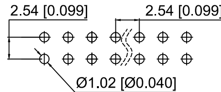
PCB Hole Layout
