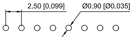
PCB Layout
