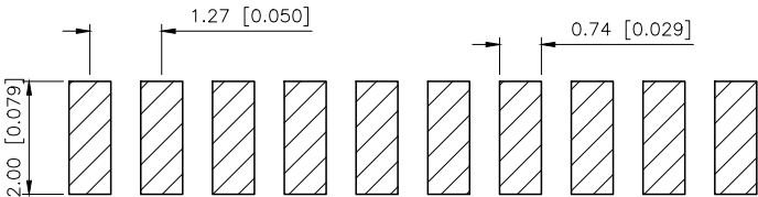
PCB_LAYOUT
