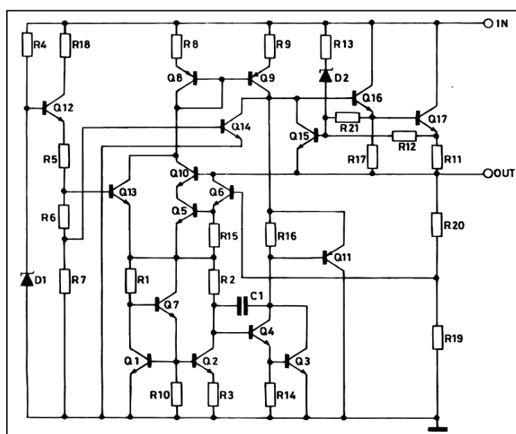
Figure 2:Schematic Diagram
