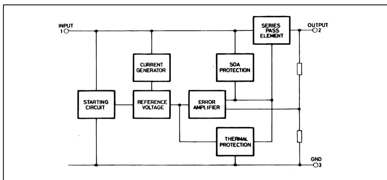
Figure 1: Schematic Diagram
