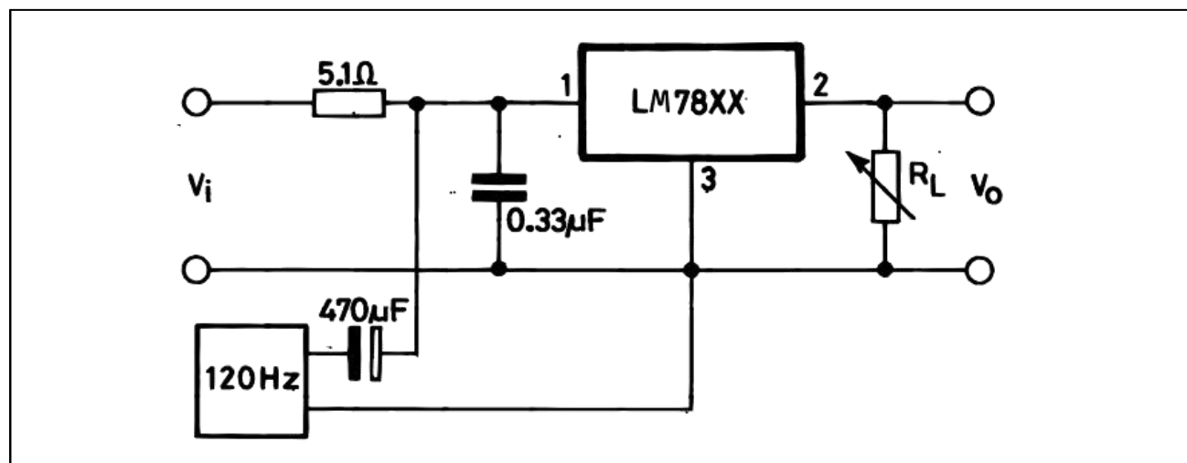
Figure 6:Ripple Rejection
