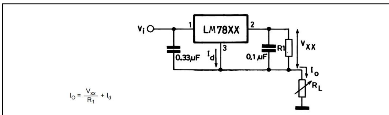
Figure 17: Current Regulator
