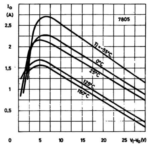
Figure 8: Peak Output Current vs Input/output Differential Voltage
