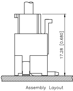
Assembly Layout
