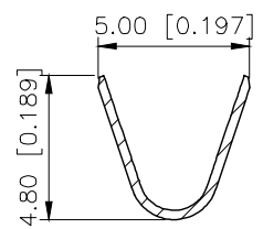
SECTION:A-A SCALE:1:1
