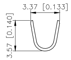
SECTION:A-A SCALE:1:1
