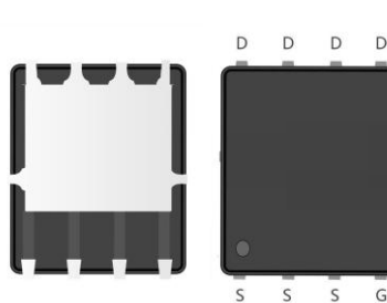
PDFN5X6-8L view
