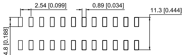
PCB LAYOUT
