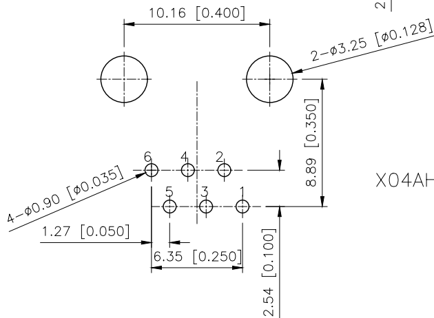
RECOMMENDED PCB LAYOUT VIEWED FROM COMPONENT SIDE
