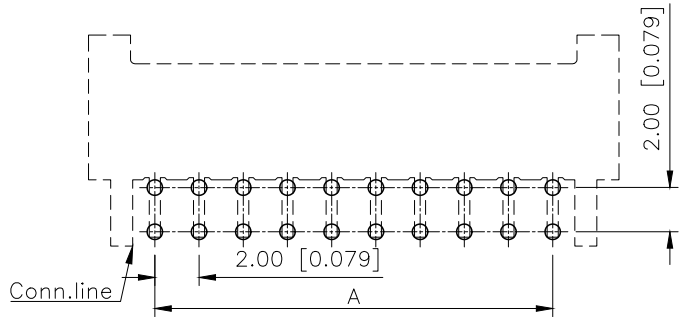
PCB LAYOUT
