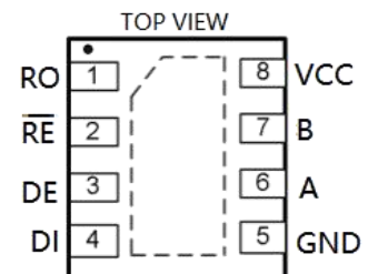
DFN-8 3*3
