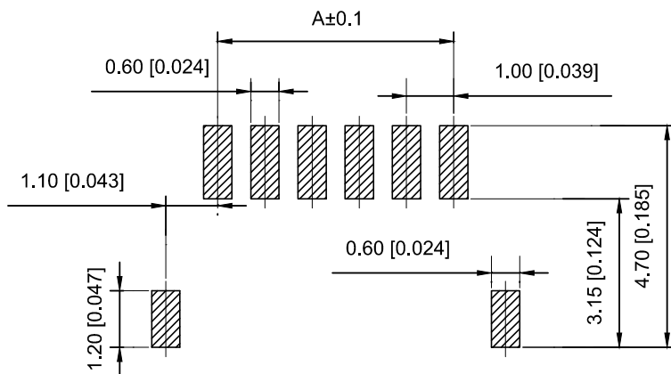
Recommended PCB hole Layout Top view(Tolerance±0.1)
