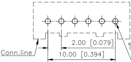
PCB LAYOUT
