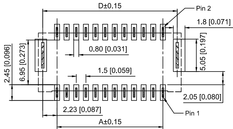
Recommended PCB Layout Tolerance:±0.05
