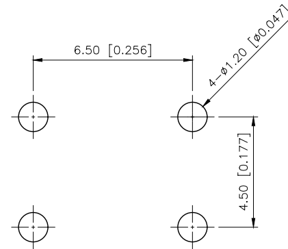
PCB.WELDING DRAWING
