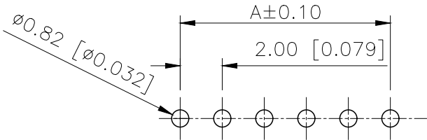
PCB LAYOUT
